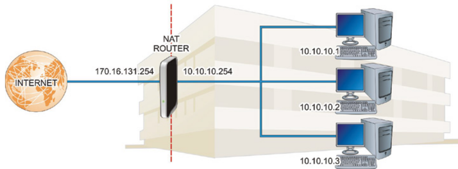
FIGURE 20.1 NAT Configuration
