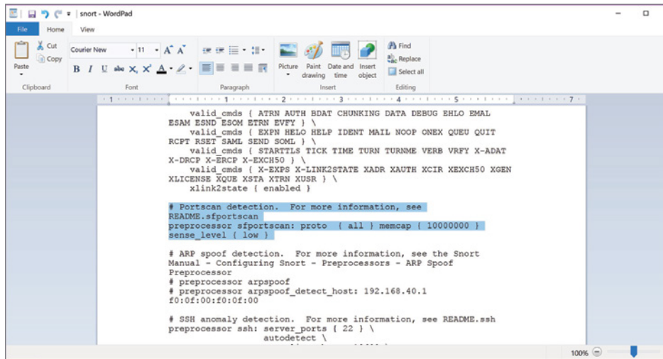
FIGURE 14.23 Enable Portscan
