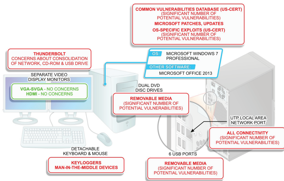
FIGURE 10.2 Known Vulnerabilities
