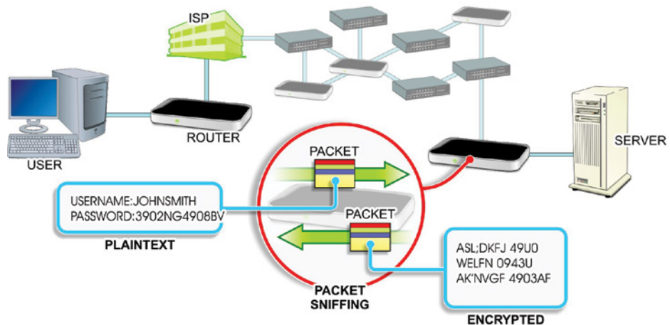
FIGURE 22.2 Viewing Credentials
