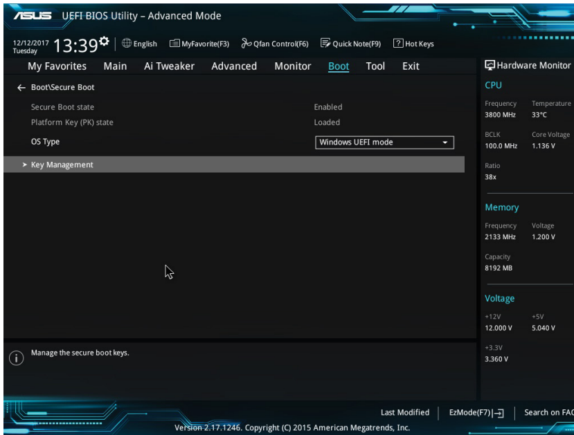
FIGURE 7.27 Key Management
