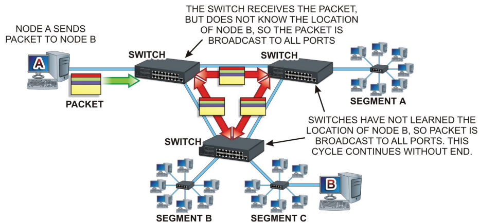
FIGURE 24.4 Broadcast Storm
