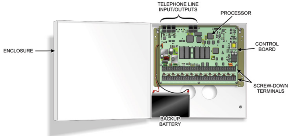
FIGURE 4.2 Control Box with Panel and Battery
