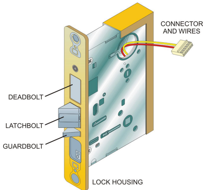
FIGURE 2.6 Electronic Deadbolt
