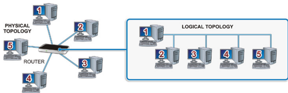
FIGURE 12.5 Logical Topologies
