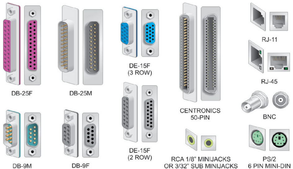
FIGURE 7.13 Typical IO Port Connectors
