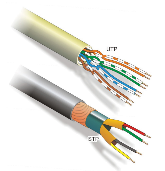
FIGURE 16.1 UTP and STP Cabling
