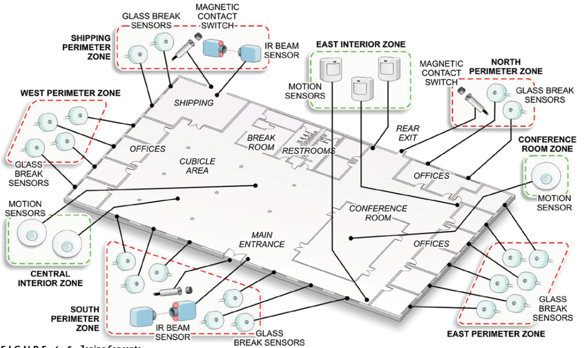
FIGURE 4.5 Zoning Concepts
