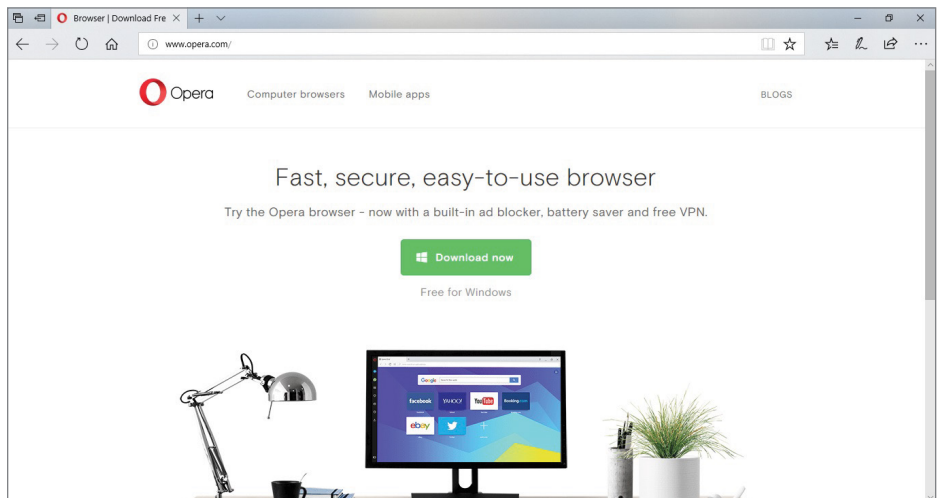
FIGURE 21.15 Viewing www.opera.com
