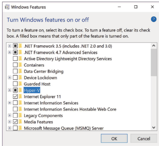
FIGURE 20.9 Enabling Hyper-V
