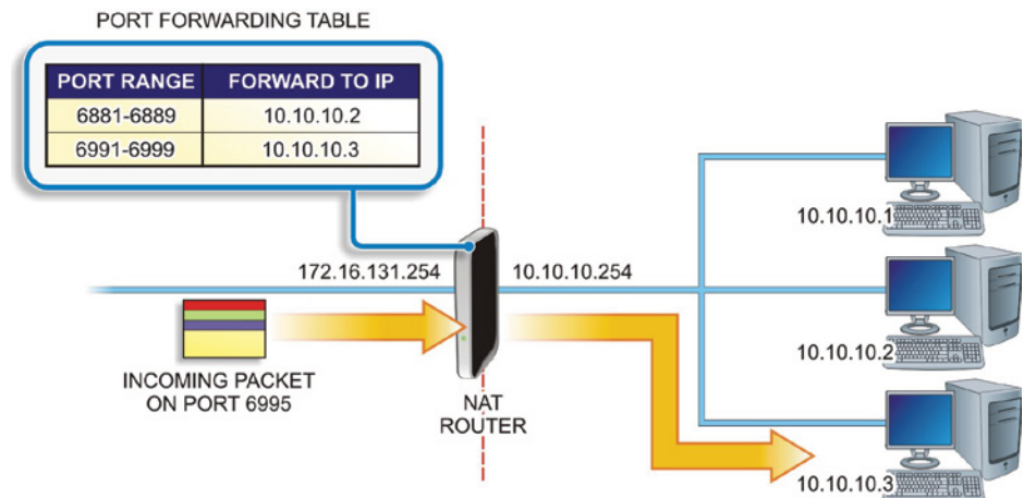
FIGURE 20.3 Port Forwarding
