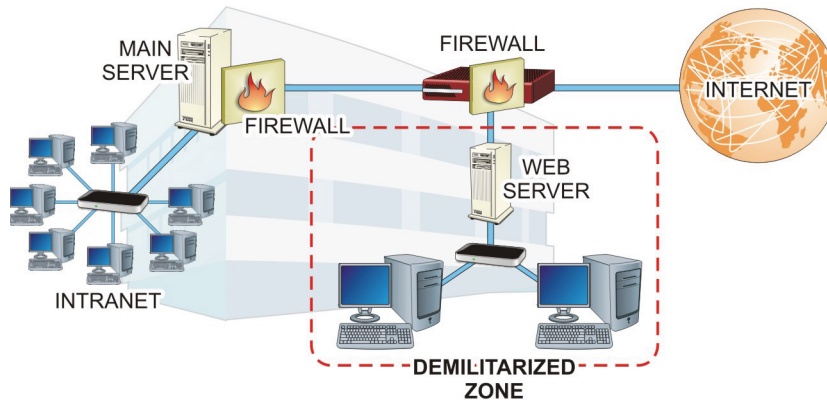
FIGURE 21.10 ADMZ
