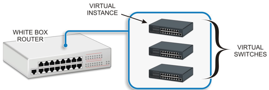
FIGURE 20.5 Virtual Instances
