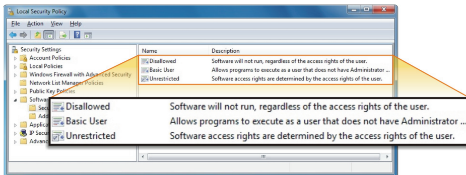
FIGURE 24.15 Security Levels
