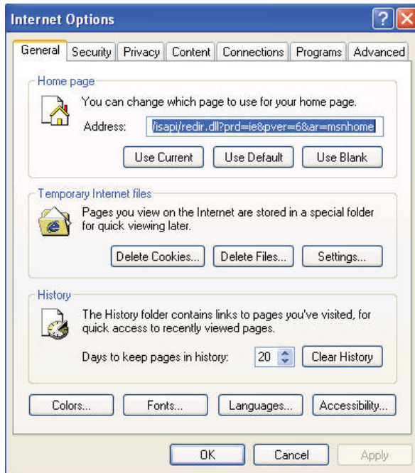
FIGURE 9.3 Internet Options
