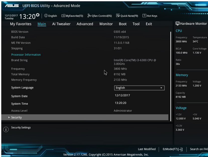
FIGURE 7.22 Security Settings
