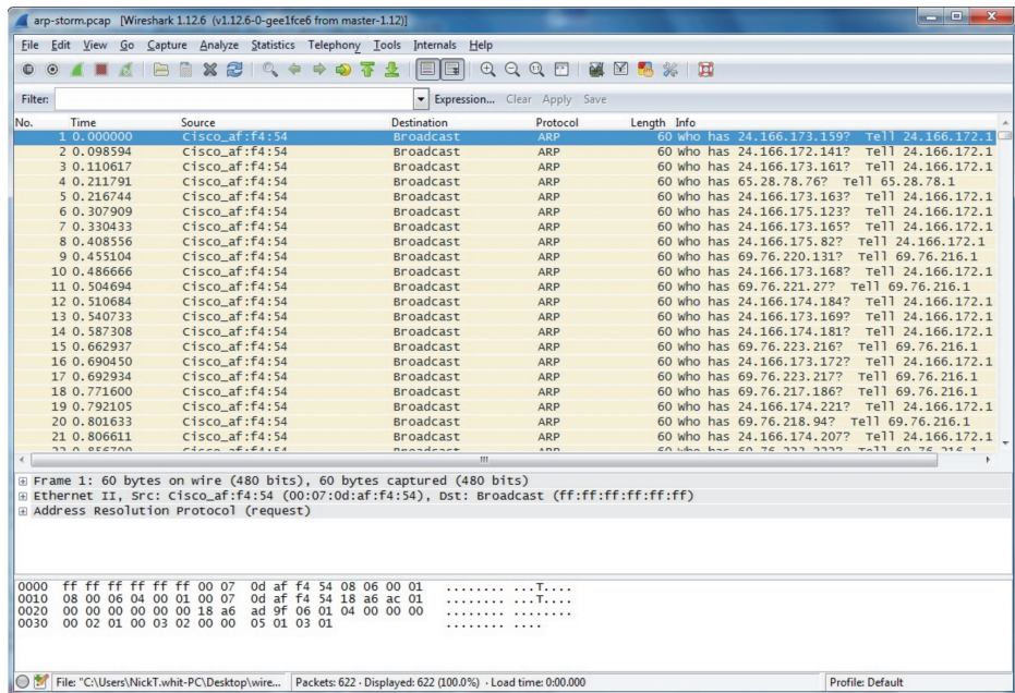
FIGURE 23.18 Arp-Storm Example
