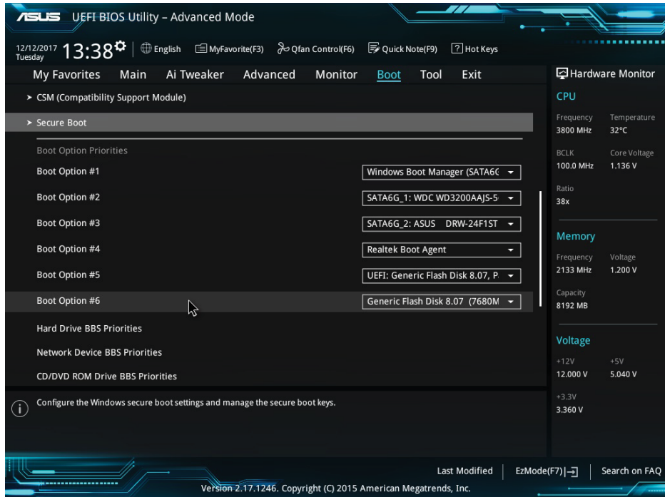
FIGURE 7.26 Secure Boot
