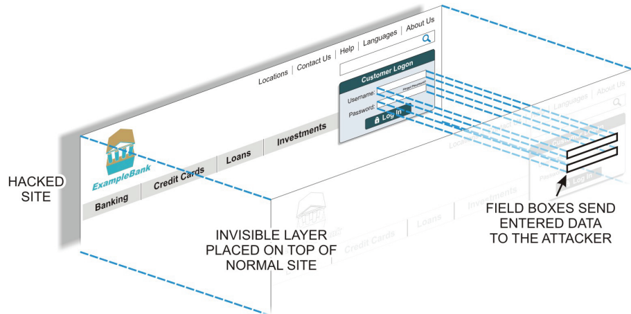
FIGURE 24.7 Clickjacking
