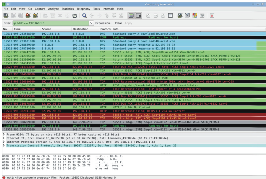
FIGURE 23.6 Wireshark
