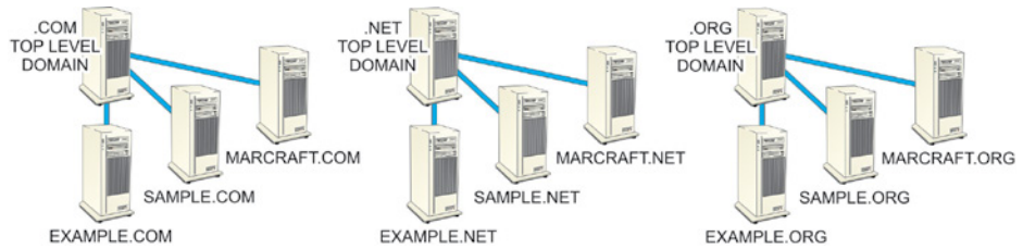
FIGURE 19.5 TLD Organization
