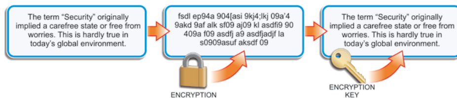
FIGURE 8.15 Data Encryption
