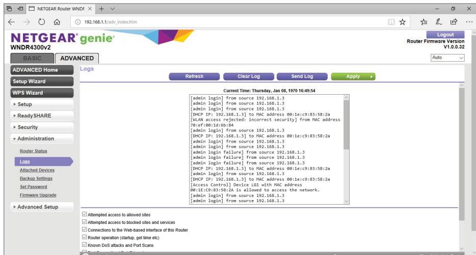
FIGURE 16.8 The Logs
