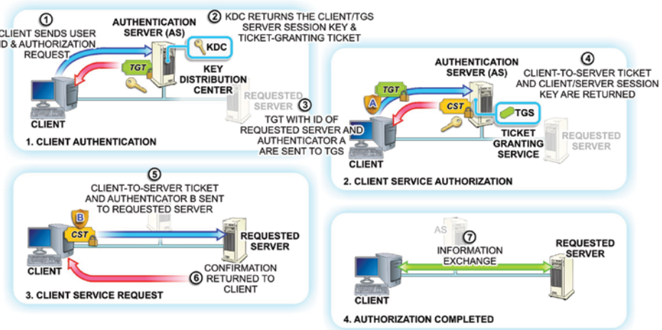
FIGURE 22.1 Kerberos Authentication
