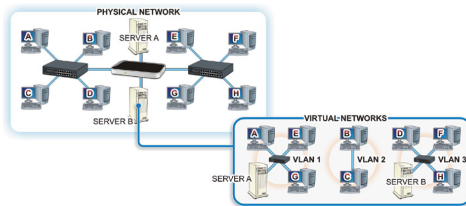
FIGURE 20.6 AVLAN
