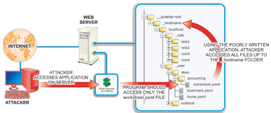
FIGURE 8.5 Directory Traversal
