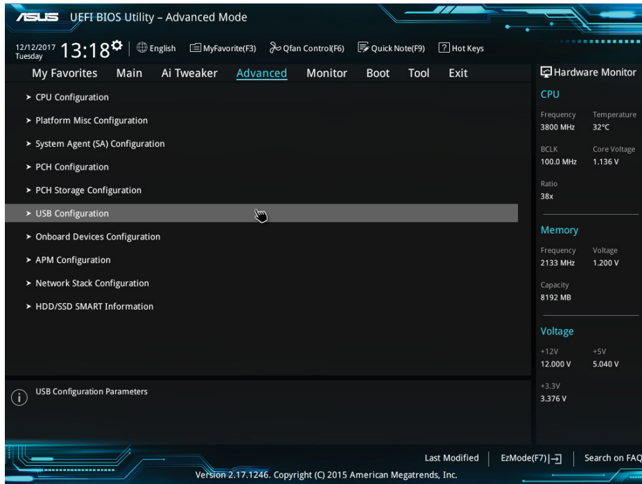
FIGURE 7.19 USB Configuration
