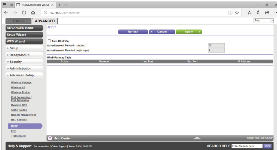
FIGURE 16.11 Disabling UPnP
