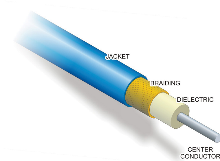
FIGURE 16.2 Coaxial Cable
