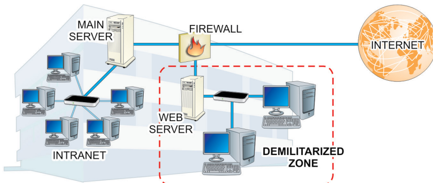
FIGURE 21.11 A Single-Firewall DMZ
